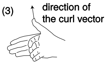
a / The div-meter, 1, and the curl-meter, 2 and 3.
